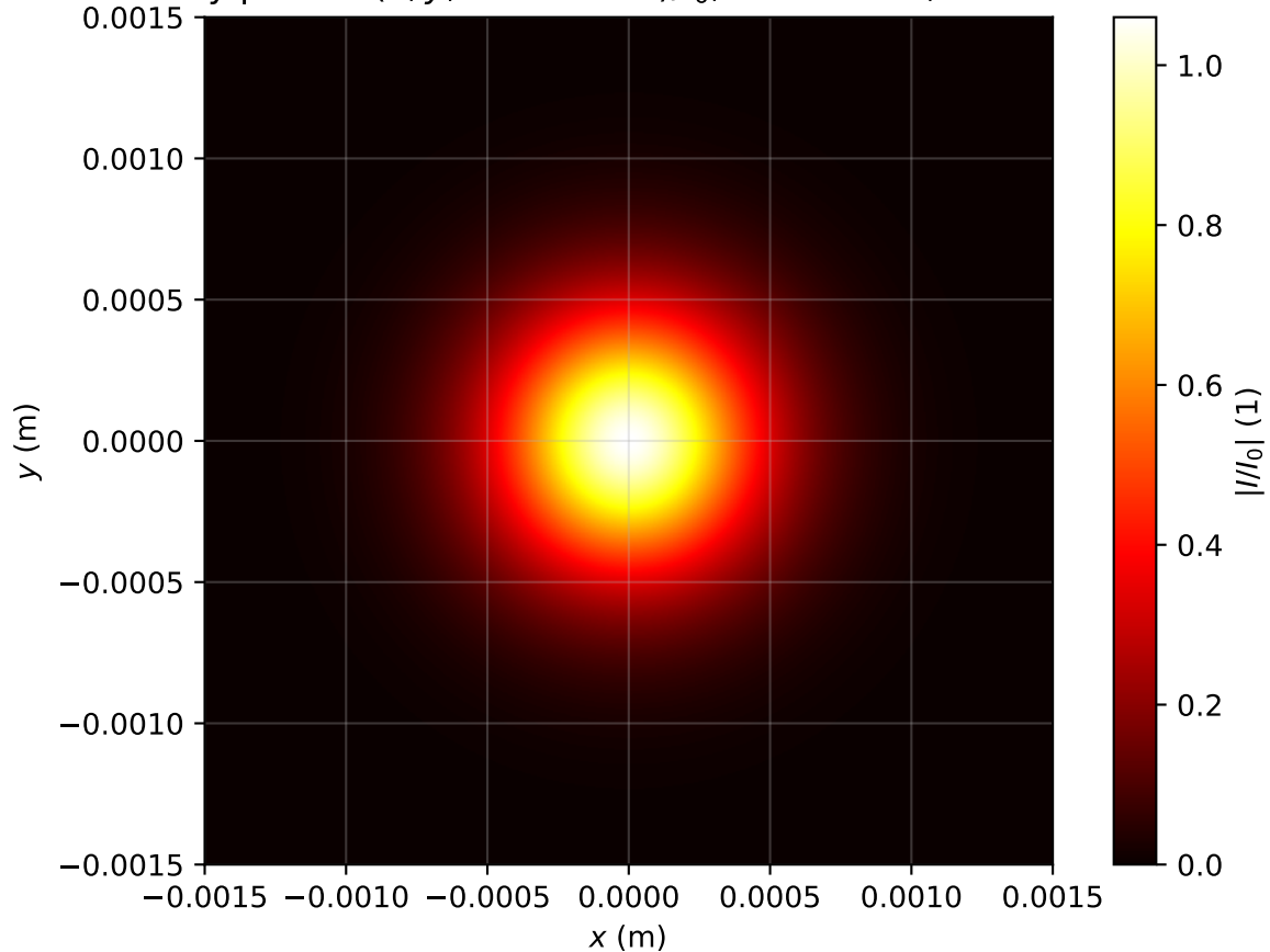
Intensity profile I(x, y, z = 0.796m)/I_0 , P_{in}=0.5P_{cr} , artificial time
